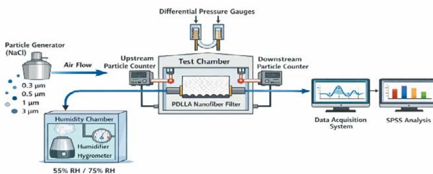
Fig. 1: Schematic of the experimental setup used for evaluating the filtration performance of PDLA nanofibers.
