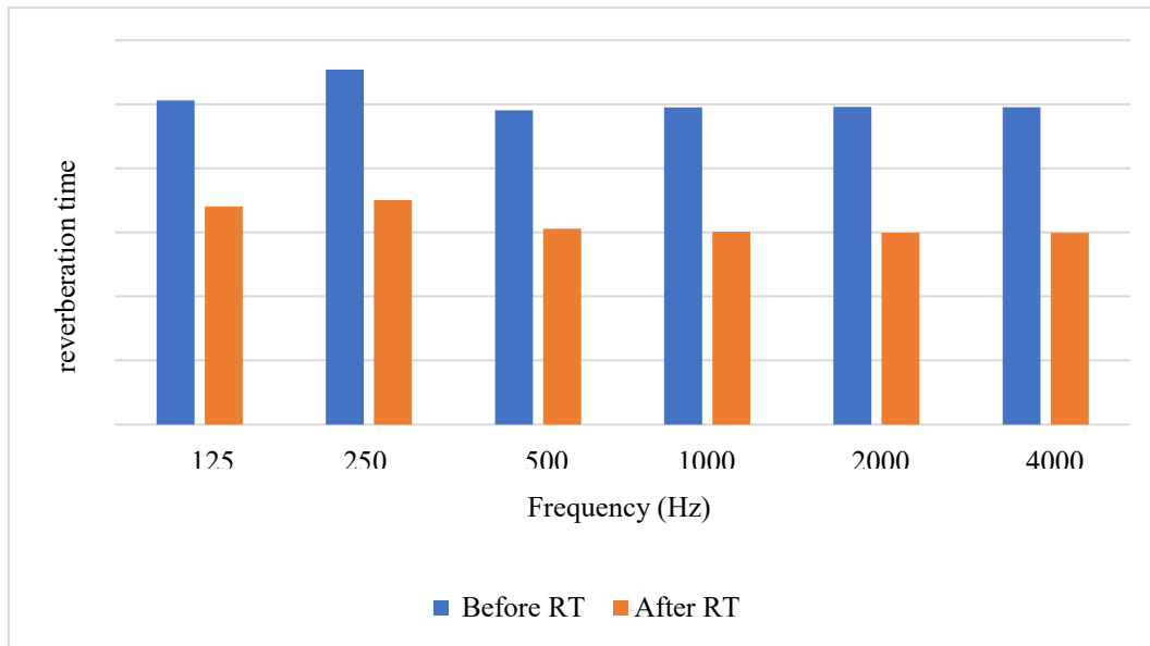
Fig. 1: Comparison of reverberation time before and after acoustic intervention at frequencies from 125 to 4000 Hz
