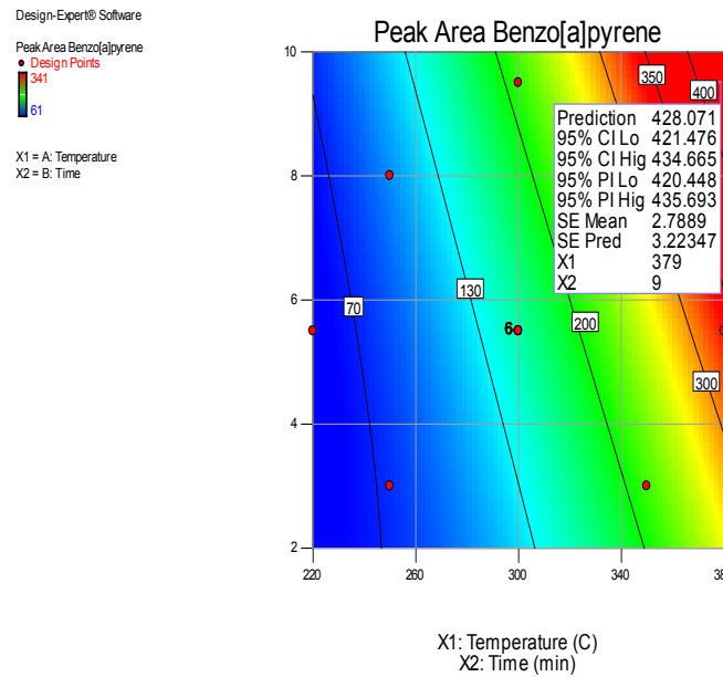
Fig. 1. Impact of temperature and time variables on the desorption of Benzo[a]pyren from needle trap
