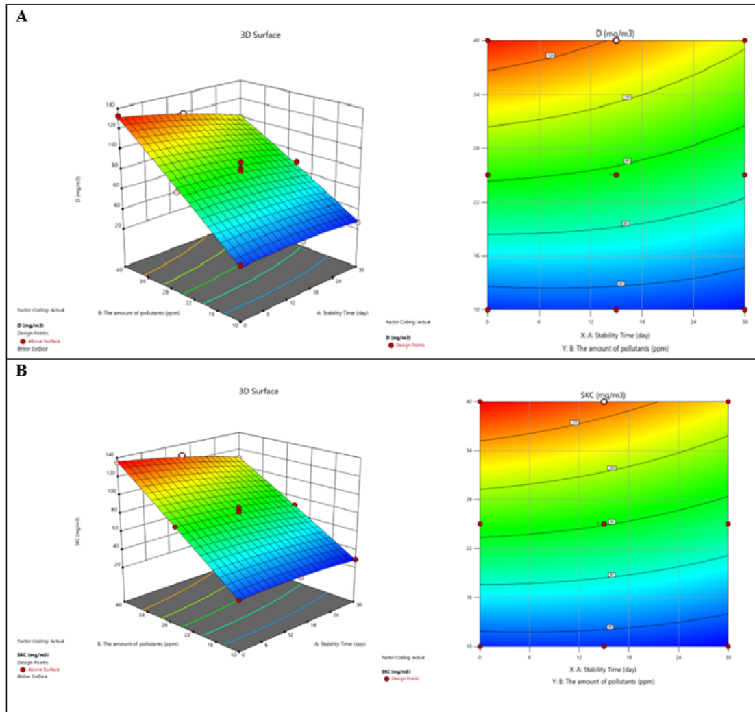
Fig. 1: Three-dimensional response surface curve illustrating the adsorption of toluene in relation to sample readsorption time and pollutant input amount for two activated carbon adsorber types: A - domestically manufactured, and B - commercial (SKC) activated
