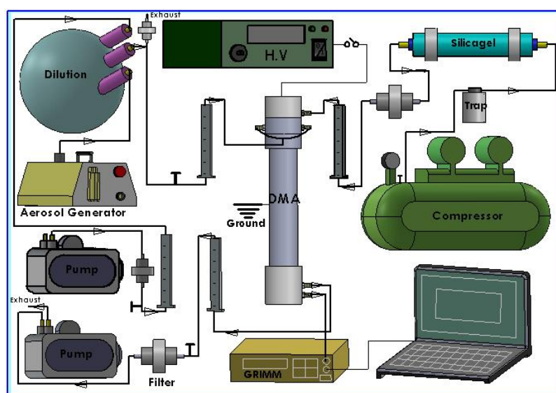
Fig. 1. Laboratory layout and equipment used in the study
