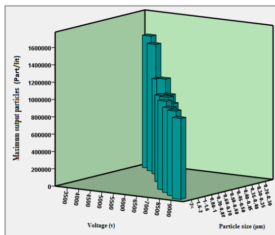
Fig. 2. Maximum output particles of DMA devices per voltage and particle size
