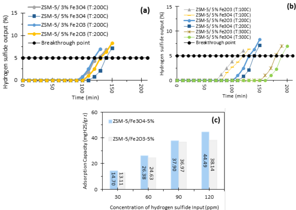
Fig. 5. (a) Catalytic substrate breakthrough curve with different loading percentages of iron nanoparticles (Temperature:200 °C – Flow 1 lit/min – concentration 60 ppm). (b) The breakthrough curve of the catalyst substrates at different reactor temperatures (Temperature:100, 200, 300 °C – Flow 1 lit/min – concentration 60 ppm). (c) Adsorption capacity of catalytic substrates with optimum iron nanoparticle loading percentage and optimum temperature nanoparticles (Temperature:300 °C – Flow 1 lit/min – concentration 30, 60, 90, 120 ppm).
